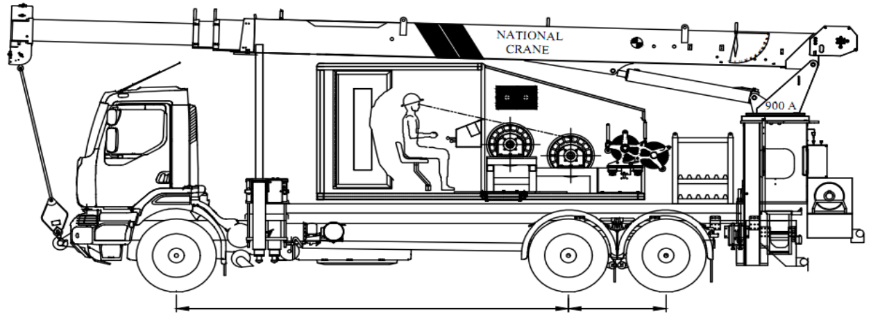
SIDE VIEW
